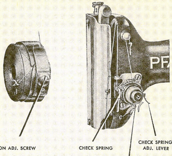
UPPER TENSION ADJ. NUT
