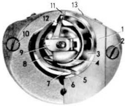
Fig. 7 Oscillating shuttle
